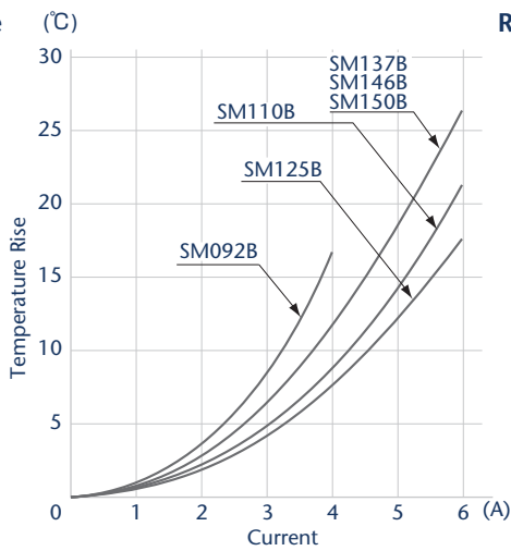
Temperature Rise
