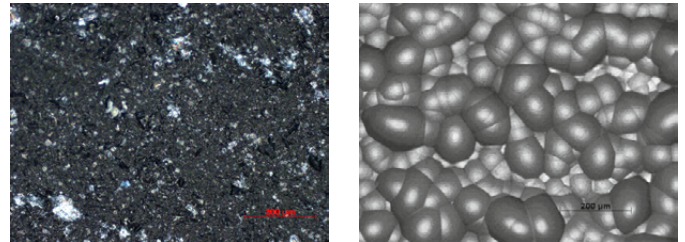
Figure 2: Surfaces of ZERODUR®, Pictured width ca. 0.9 mm Left: Ground with D151 bonded diamond grains. Right: strongly etched
