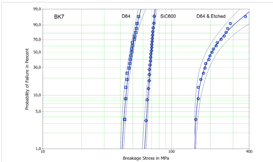
Figure 9: Breakage stress data sets for the optical glass BK7 with three different surface conditions: Ground with bonded diamond grain D64 with maximum grain size of 64 \mu\text{m} , lapped with silicon carbide fine grain SiC600 with 19 \mu\text{m} maximum grain size and D64 ground and subsequently etched. Three parameter Weibull distribution fitted and given with 90% confidence bounds.
