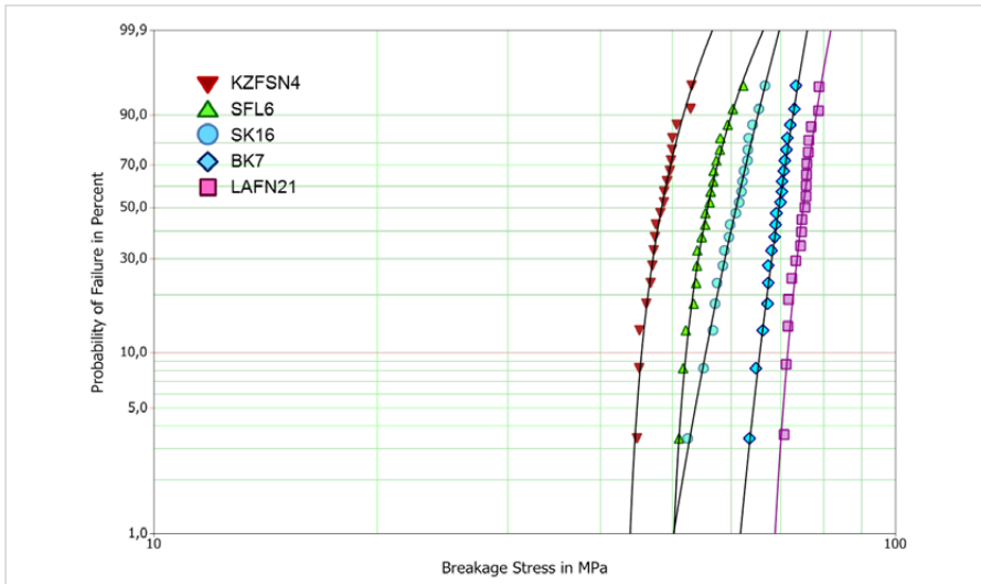
Figure 8: Breakage stress data sets for some optical glasses lapped with silicon carbide fine grain SiC600 with maximum grain size of 19 \mu\text{m} . The lines represent three parameter Weibull distributions fitted to the data sets.
