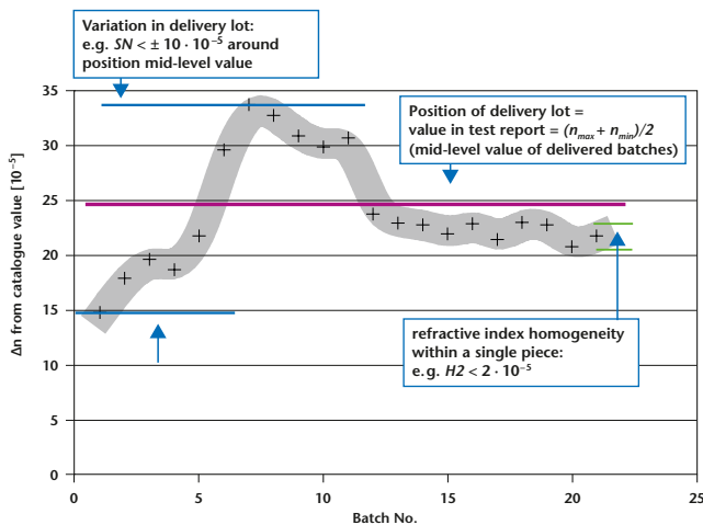
Fig. 6: Refractive index variation from within a production sequence.
