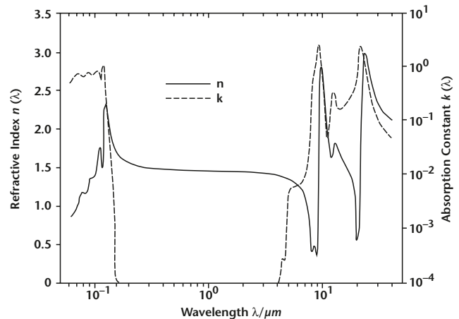
Fig. 1: Measured optical constants of fused silica (SiO 2 glass) [1].
