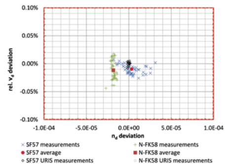
Fig.9: Reproducibility of V-block refractometer. Red box indicates the tolerance step. In order to give an impression of the deviation size we added the tolerance range of SCHOTT's best commercially available quality step 0.5 (red dashed line).
