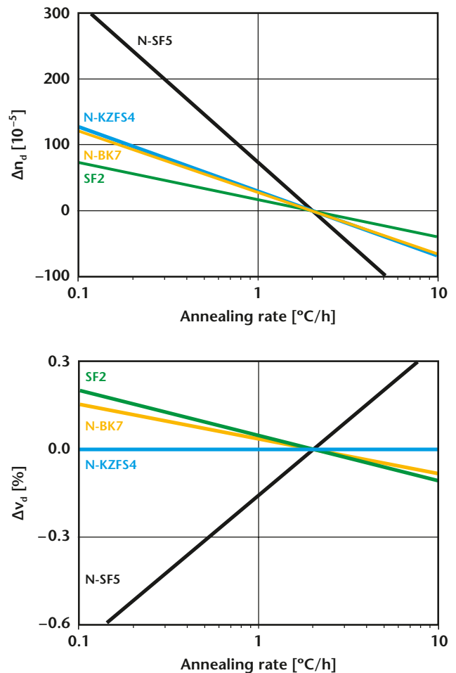
Fig. 4: Dependence of refractive index n_d (a: upper) and Abbe number v_d (b: lower) on the annealing rate for several glass types. Reference annealing rate is 2 °C/h [3].
