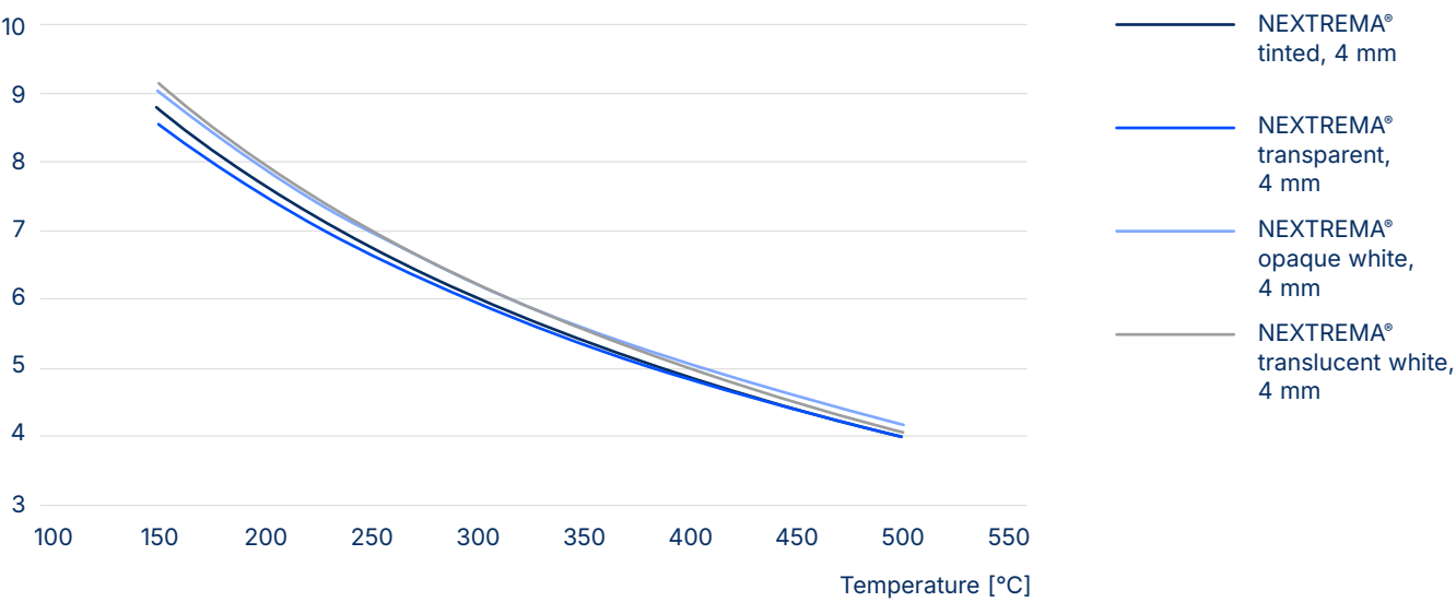
Specific electrical volume resistance at different temperatures for selected NEXTREMA® types (log ρ [Ω · cm]), shown as representative curves.
