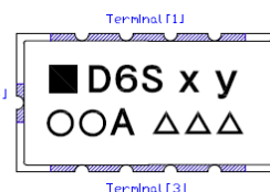
Fig.1 Terminal position
