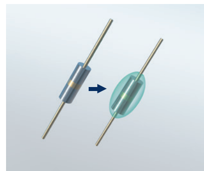
Protective passivation glass
