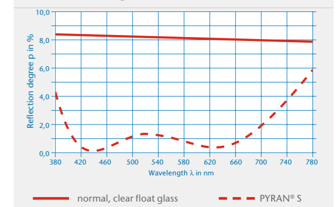
Comparison of reflection of anti-reflective PYRAN® S and normal, clear float glass
