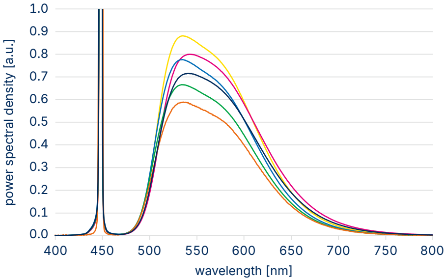
Emission spectrum
