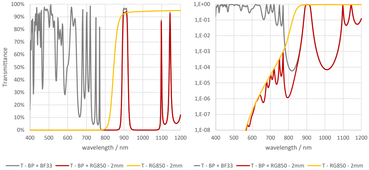
Figure 5: The graphs show the transmittance of different filter elements that can be combined. On the left is a linear scaling and the right shows logarithmic scaling of the ordinate. The grey graph depicts the interference filter design while the orange curve is the filter glass RG850. The red graph shows the result: very low transmittance from 400 nm to 900 nm, a high transmittance area from 900 to 920 nm, and nice blocking from 920 to 1050 nm.
