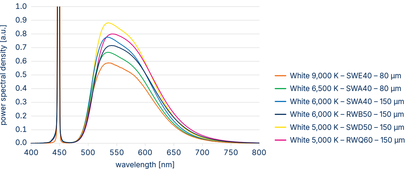
Emission spectrum
