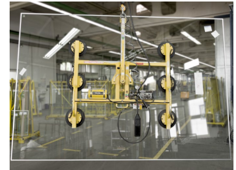
Vacuum suction cups must be evenly distributed across the surface of the glass pane.
